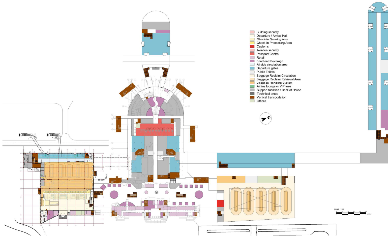
FIGURE 10 FUNCTIONAL LAYOUT 2052 LEVEL 1
